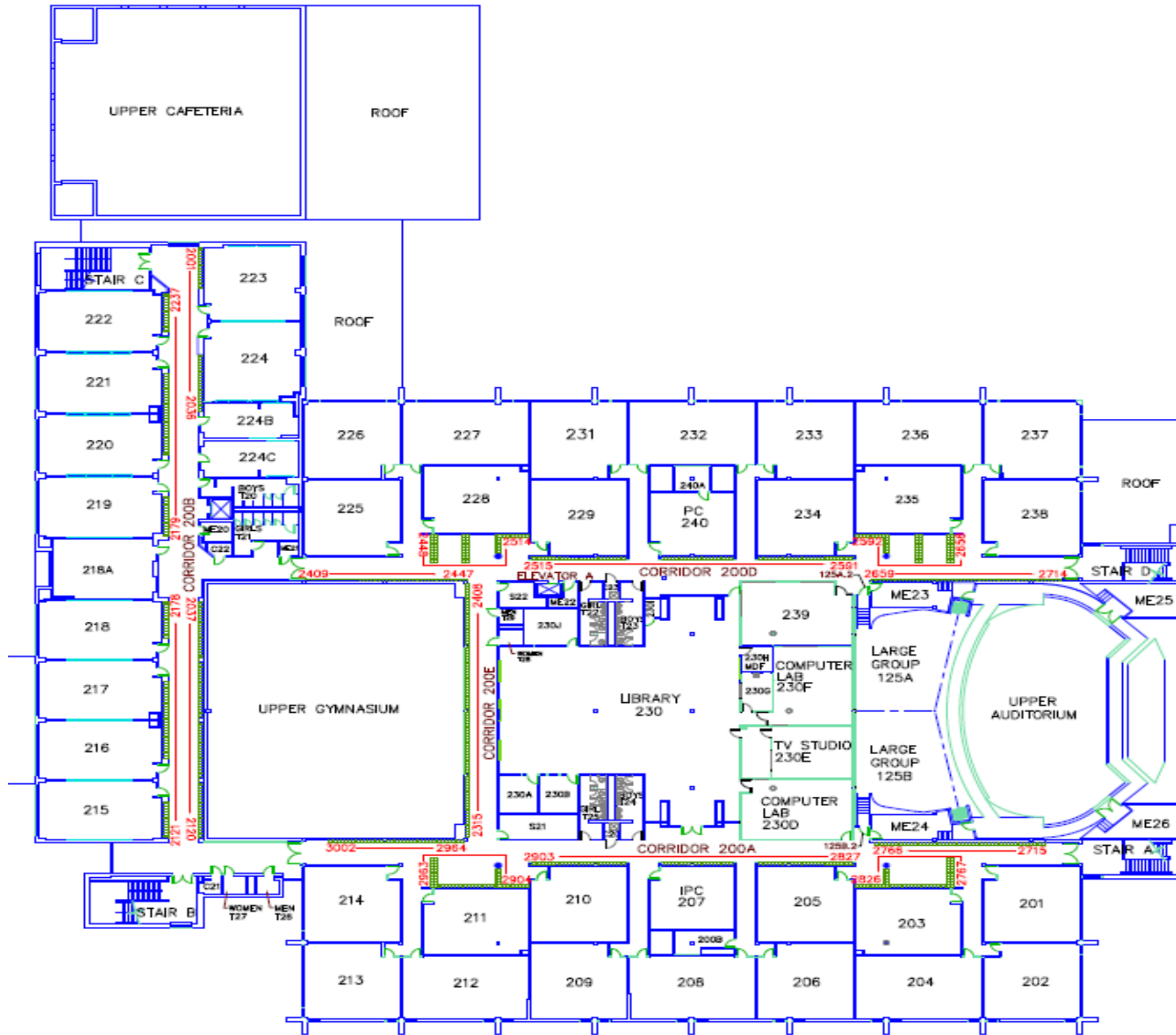
HOLICONG MIDDLE SCHOOL SECOND FLOOR PLAN
